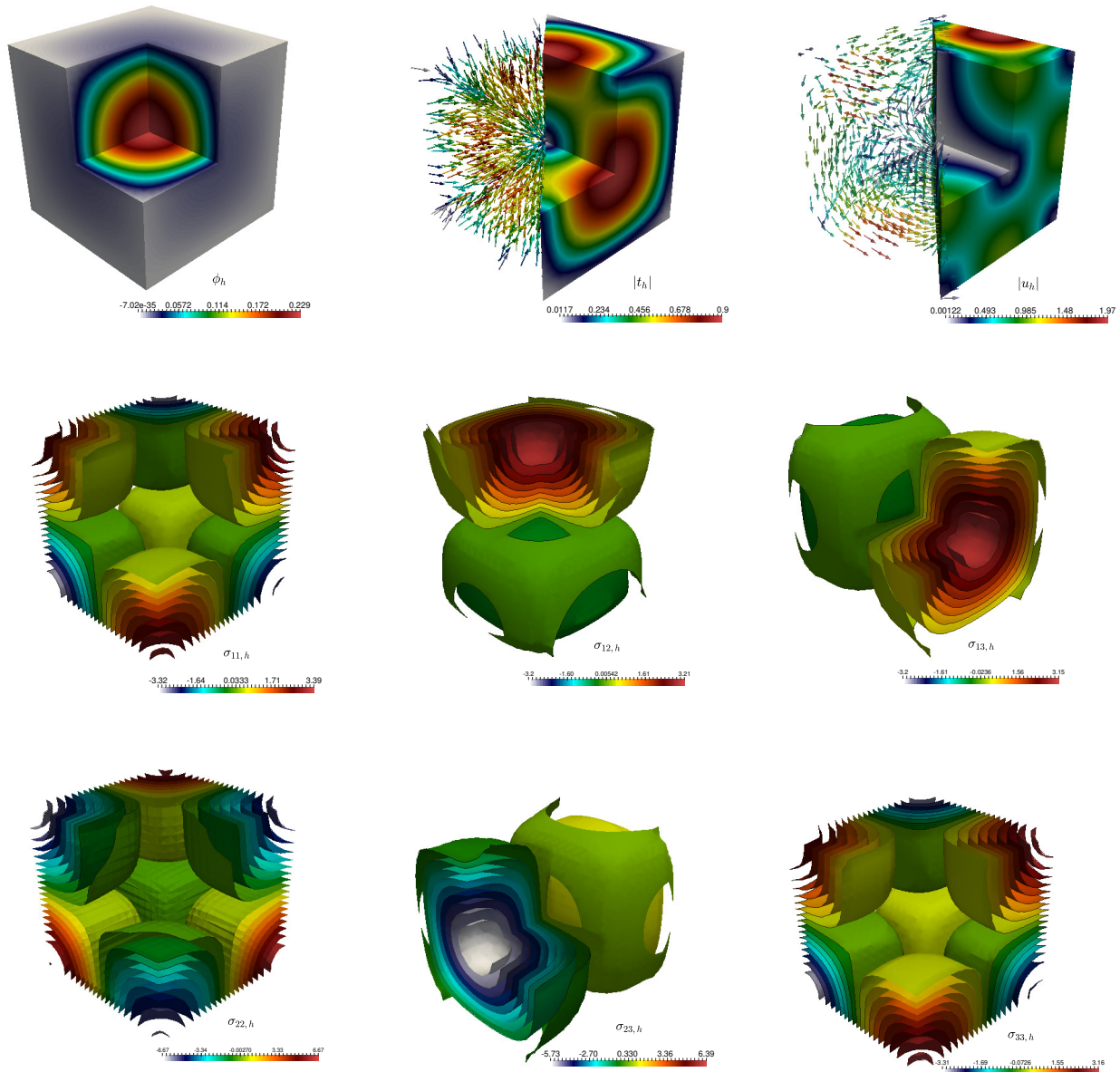
Figure 6.0.4: Numerical Results for Example 4: From left to right and from up to down: approximation of scalar field concentration \phi_h , gradient of concentration t_h , velocity components u_h , stress components \sigma_h . Snapshots obtained from a simulation with 369 094 DOF.
