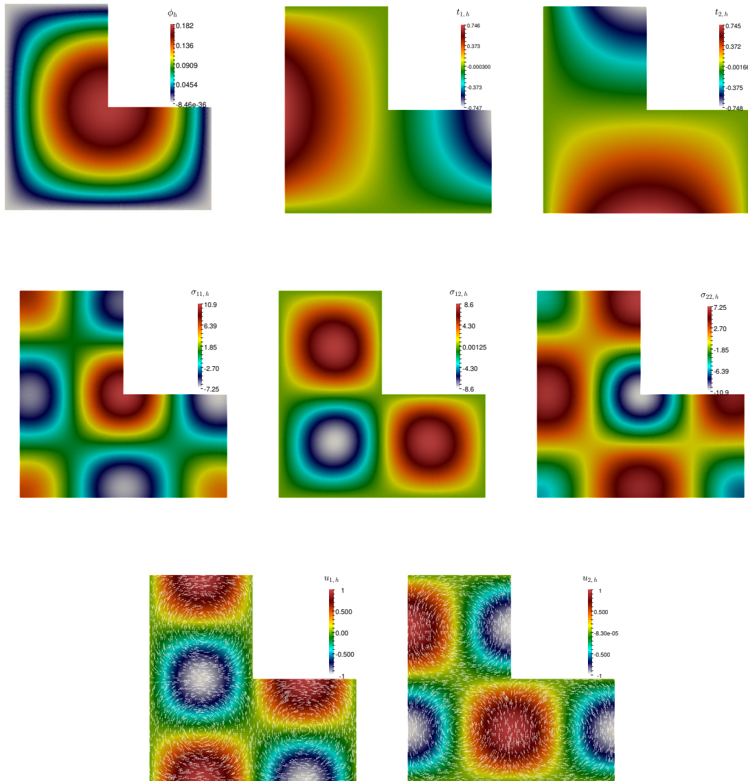
Figure 6.0.2: Numerical Results for Example 2: From left to right and from up to down: approximation of scalar field concentration \phi_h , gradient component of concentration t_h , stress components \sigma_h and velocity components \mathbf{u}_h . Snapshots obtained from a simulation with 230 321 DOF.
