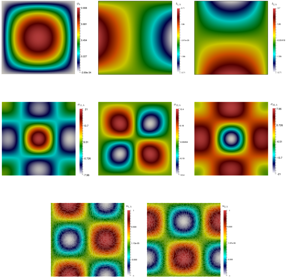
Figure 6.0.1: Numerical Results for Example 1: From left to right and from up to down: approximation of scalar field concentration \phi_h , gradient component of concentration t_h , stress components \sigma_h and velocity components u_h . Snapshots obtained from a simulation with 54 885 DOF.
