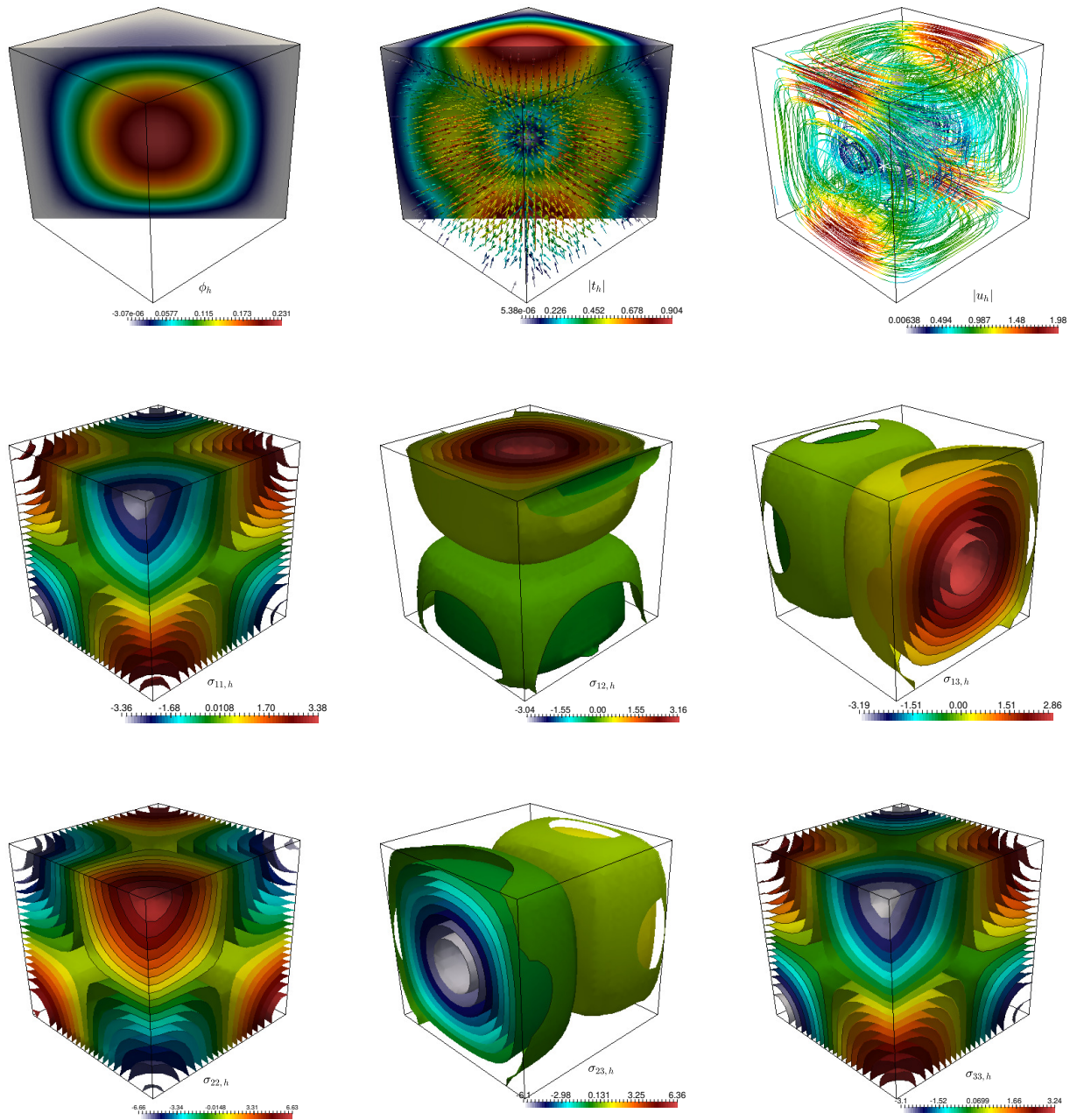
Figure 6.0.3: Numerical Results for Example 3: From left to right and from up to down: approximation of scalar field concentration \phi_h , gradient of concentration t_h , velocity u_h and stress components \sigma_h . Snapshots obtained from a simulation with 493 358 DOF.
