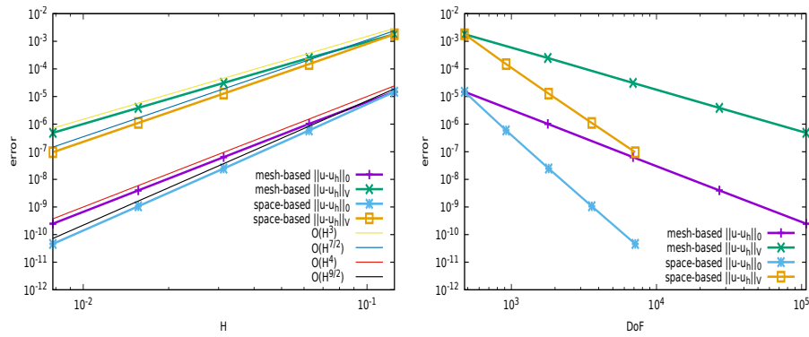
Fig. 5 Comparison between mesh-based and space-based convergences on L-shaped elements for k = 2 in the L^2 and V norms with respect to H (left) and the DoF (right).
