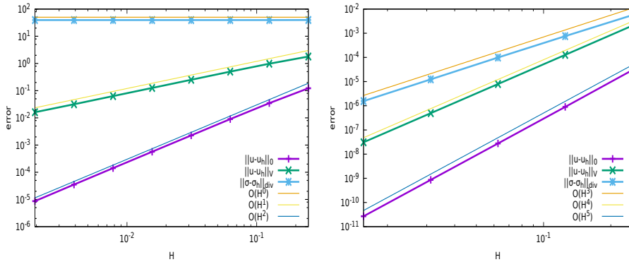
Fig. 2 The mesh-based convergence history on quadrilateral elements for k = 0 (left) and k = 3 (right).
