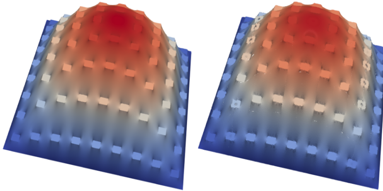
Fig. 10 The 9 \times 9 inclusions test case. Elevation of the reference solution (left) and the MHM's solution obtained on a 32 L -shaped element mesh (right) with DoF = 624 .
