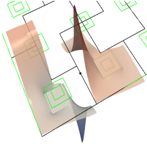
Fig. 8 A multiscale basis function associated with a degree of freedom (black dot) on a L -shaped mesh with the \mathbb{P}_1(F) \times \mathbb{P}_2(\mathfrak{T}) element. We observe the influence of the high-contrast coefficients on the basis function.
