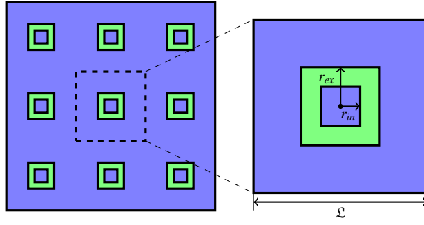
Fig. 7 Sketch of the heterogeneous diffusive media with 3 \times 3 inclusions. Here r_{in} = \frac{1}{32} , r_{ex} = \frac{1}{16} , L = \frac{1}{3} , and the diffusive coefficient is \kappa = 1 (blue) and \kappa = 10^5 (green).
