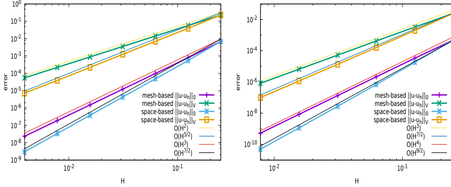
Fig. 3 Comparison between mesh-based and space-based convergences on quadrilateral elements for k = 1 (left) and k = 2 (right) in the L^2 and V norms.
