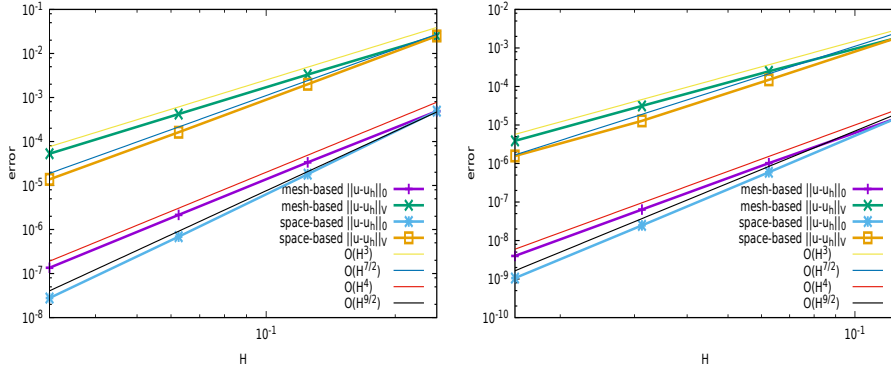
Fig. 6 Comparison between mesh-based and space-based convergences on quadrangular (left) and L-shaped elements (right) using the \mathbb{P}_{k+1}(F) \times \mathbb{P}_{k+1}(\mathcal{T}) element with k = 1 in the L^2(\Omega) and H^1(\mathcal{P}) norms.
