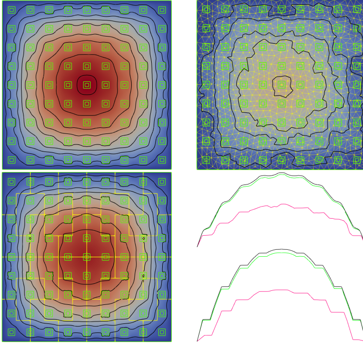
Fig. 11 The 9 \times 9 inclusion test case: Comparison between the reference solution (top left) and the Galerkin solution on a conform triangular mesh with DoF = 3,283 (top right), and the MHM solution (bottom left) on a non-conforming L -shaped mesh with DoF = 624 . Cross sections at x = 0.25 and x = 0.5 (bottom right) show that the MHM method improves the accuracy when compared to the Galerkin method with polynomial basis functions.
