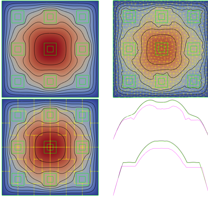
Fig. 9 The 3 \times 3 inclusion test case: Comparison between the reference solution (top left) and the Galerkin's solution on a conforming triangular mesh with DoF = 3,283 (top right) and the MHM's solution (bottom left) on a non-conforming L -shaped mesh with DoF = 624 . Cross sections at x = 0.25 and x = 0.5 (bottom right) are shown illustrating the lack of accuracy of the Galerkin method compared to the MHM solution.
