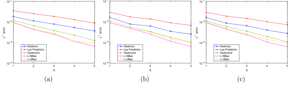
Figure 2: Test 1. Initial condition (4.1). Approximate \mathbf{L}^1 -error for different numerical schemes with: (a) constant kernel function \omega(x) = 1/\eta , (b) decreasing kernel function \omega(x) = 2(\eta - x)/\eta^2 , (c) concave kernel function \omega(x) = 3(\eta^2 - x^2)/(2\eta^3) .
