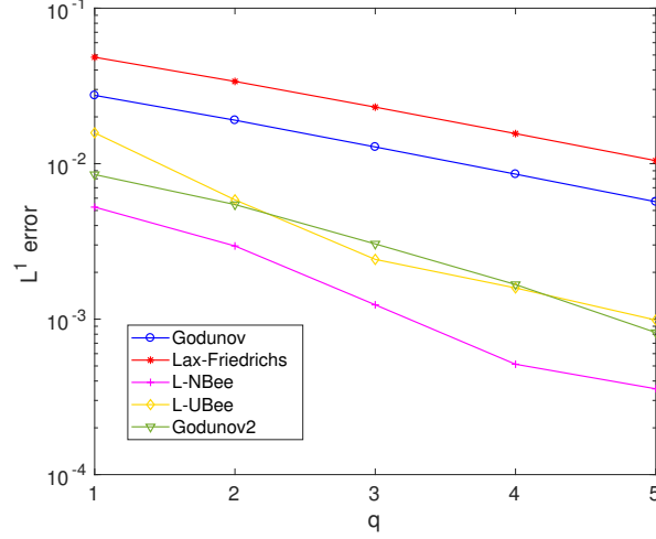
Figure 6: Test 2. Approximate total L^1 -error for different numerical schemes with the decreasing kernel functions \omega_1(x) = \omega_2(x) = 2(\eta_{1,2} - x)/\eta_{1,2}^2 , \eta_1 = 0.3 , \eta_2 = 0.1
