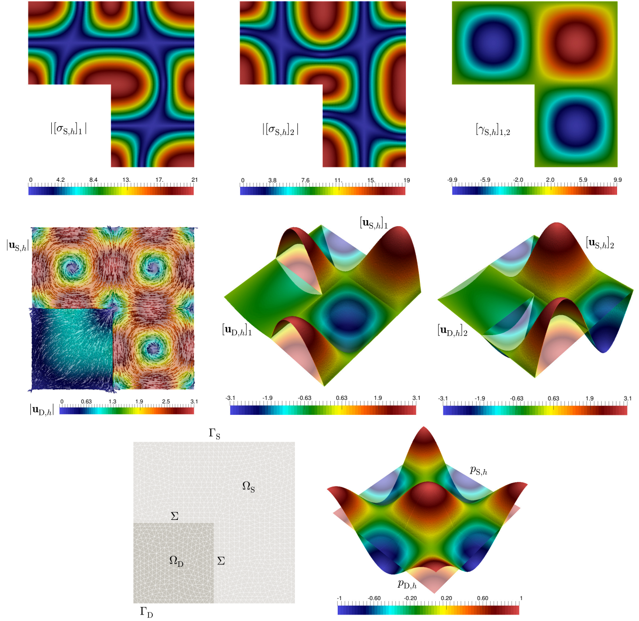
Figure 7.1: Example 1. Approximated spectral norm of the nonlinear pseudostress tensor components and the skew-symmetric part of the Navier–Stokes velocity gradient (top panel), velocity streamlines and velocity components on the whole domain (middle panel), and geometry configuration and pressure field in the whole domain (bottom panel).
