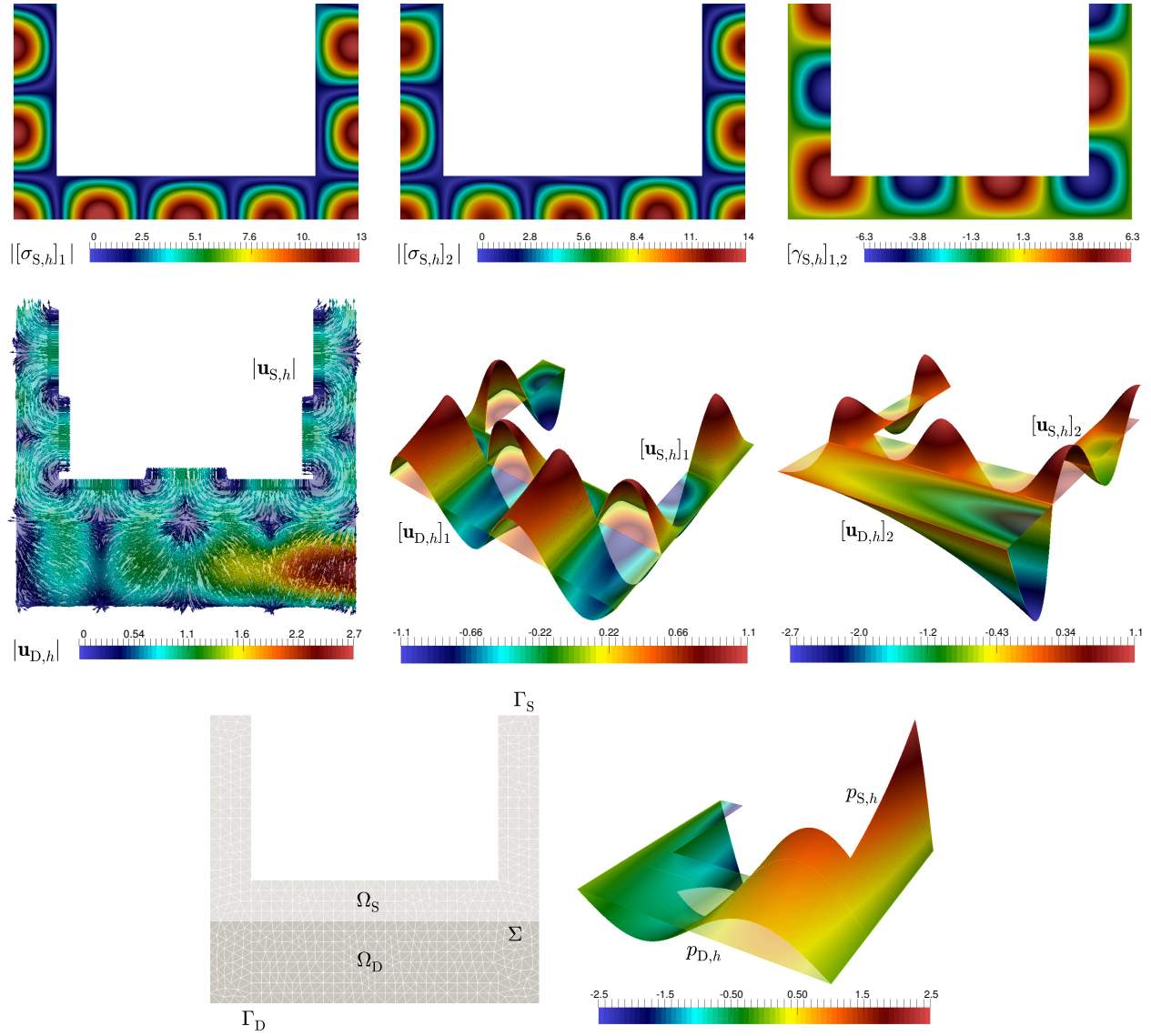
Figure 7.2: Example 2. Approximated spectral norm of the nonlinear pseudostress tensor components and the skew-symmetric part of the Navier–Stokes velocity gradient (top panel), velocity streamlines and velocity components on the whole domain (middle panel), and geometry configuration and pressure field in the whole domain (bottom panel).
