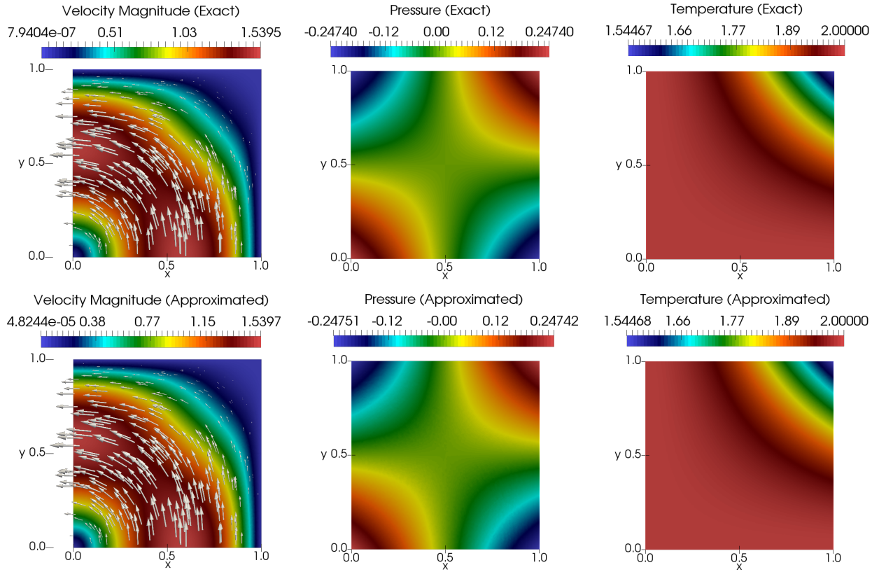
Figure 6.1: Graphical comparison of the exact solution (\mathbf{u}, p, \varphi) (upper row) and its numerical approximation (\mathbf{u}_h, p_h, \varphi_h) (lower row) for the data given in Example 1. Results calculated with 216,315 DOF and a first-order approximation (\mathbb{RT}_0 - \mathbf{P}_1 - P_0 - P_1 - P_0) .
