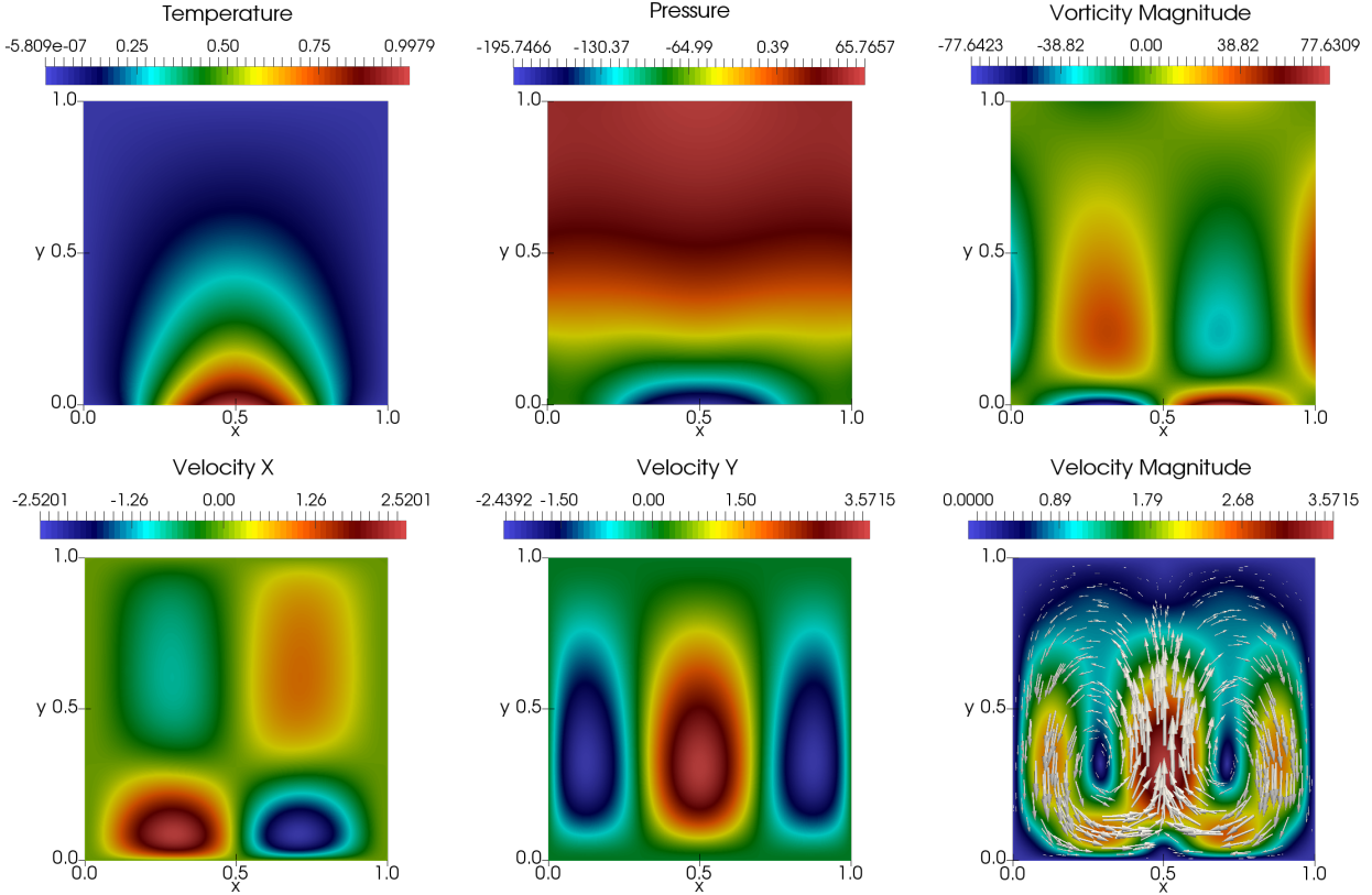
Figure 6.2: Contours of temperature, pressure and vorticity magnitude (taken as 2\gamma_{21} to coincide with the usual definition of vorticity) in the upper row, and velocity in the lower row for the data given in Example 2. Results calculated with 3,493,345 DOF and a first order approximation ( \mathbb{RT}_0 - \mathbf{P}_1 - P_0 - P_1 - P_0 ).
