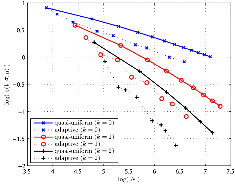
Figure 6.4: Example 4, e(t, \sigma, u) vs. N .
