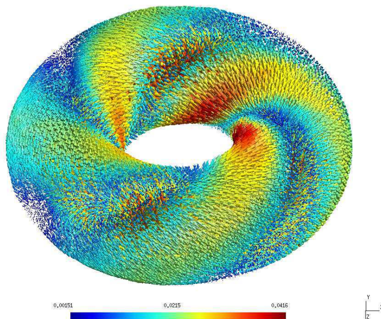
FIGURE 5. Beltrami field corresponding to the smallest positive eigenvalue.
