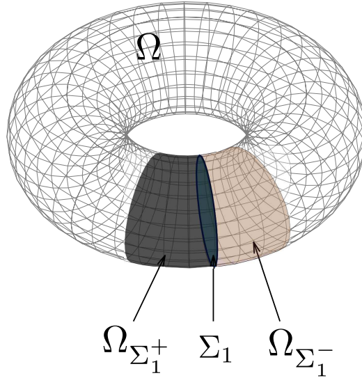
FIGURE 2. Toroidal domain for the proof of Lemma 3.12.
