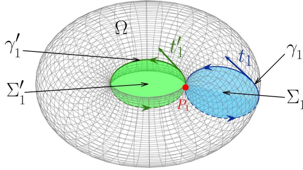
FIGURE 1. A multiply connected domain. Notation.
