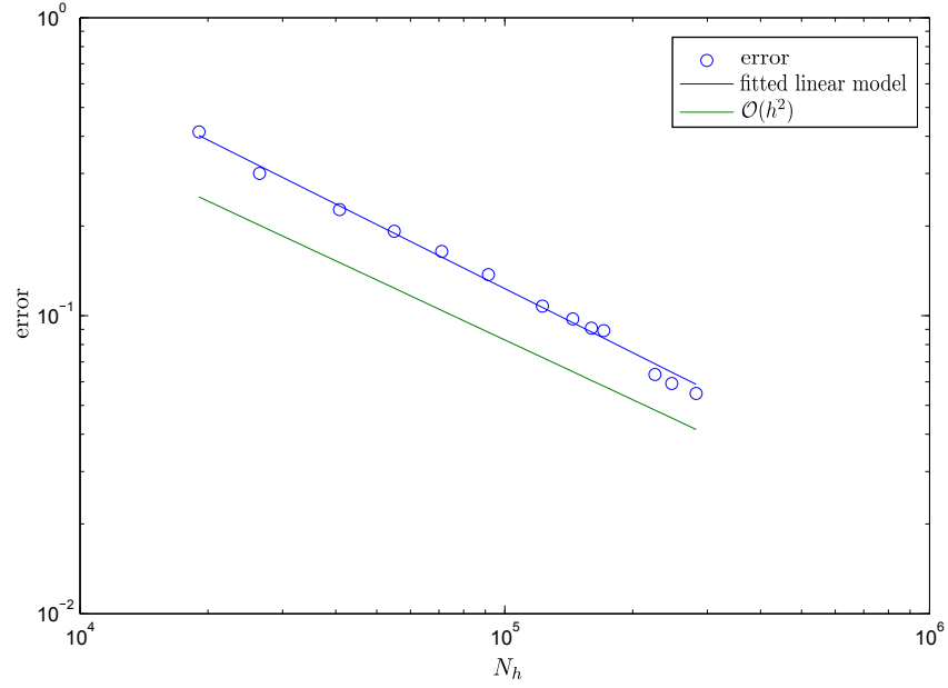
FIGURE 4. Error curve for the smallest positive eigenvalue: log-log plot of the computed error |\lambda_{h,1} - \lambda_{\text{ex}}| versus the number of tetrahedra N_h .
