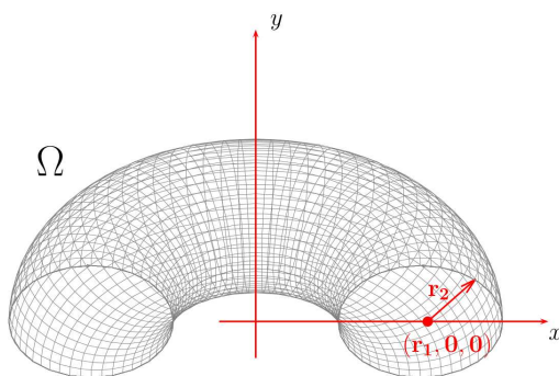
FIGURE 3. Half of the toroidal domain for the numerical test.
