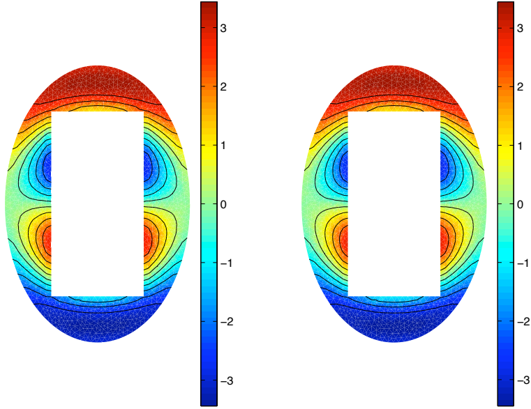
Figure 5.7: Approximate and exact real part of \sigma_{f,2} (EXAMPLE 2)
