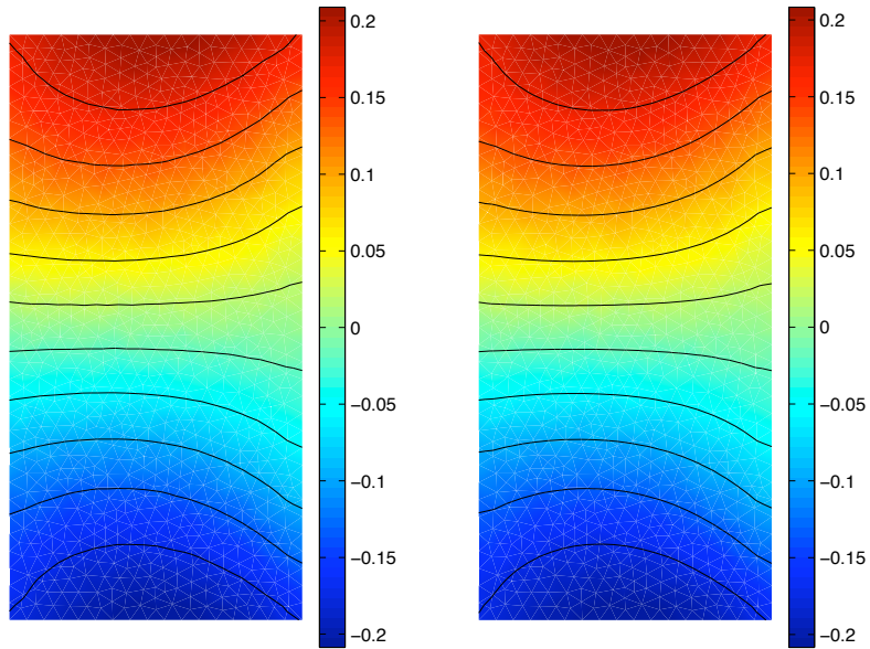
Figure 5.2: Approximate and exact real part of \sigma_{s,21} (EXAMPLE 1)
