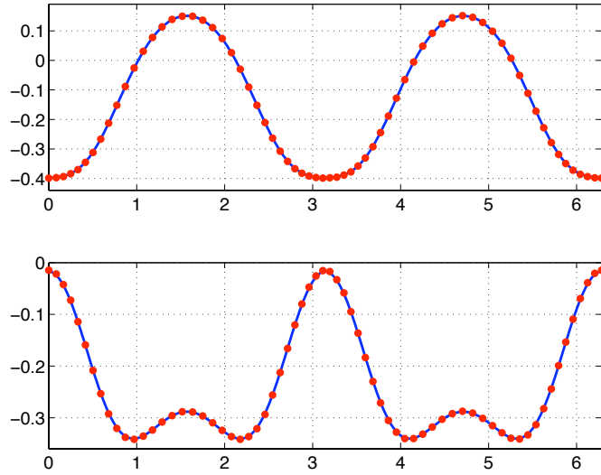
Figure 5.8: Approximate (red) and exact (blue) real and imaginary parts of \varphi_\Gamma (EXAMPLE 2)
