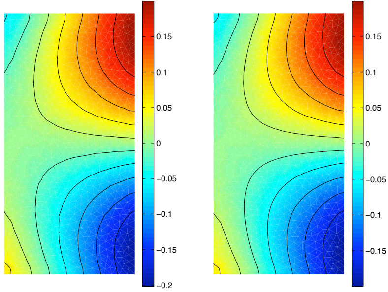
Figure 5.1: Approximate and exact imaginary part of \sigma_{s,12} (EXAMPLE 1)
