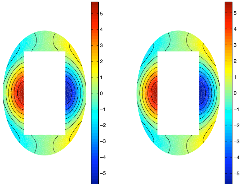
Figure 5.6: Approximate and exact real part of \sigma_{f,1} (EXAMPLE 2)
