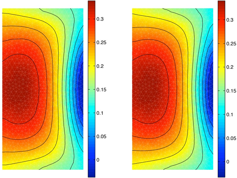
Figure 5.5: Approximate and exact imaginary part of \sigma_{s,11} (EXAMPLE 2)
