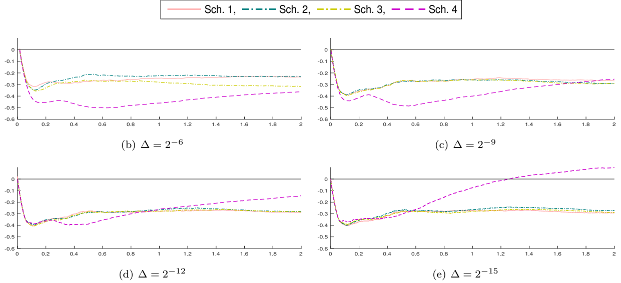
Figure 3: Computation of the Mandel-Q parameter (23) corresponding to System 4 with d = 50 and \omega_3 = 1.1\omega_2 . We use 20000 realizations of Schemes 1, 2, 3 and 4.
