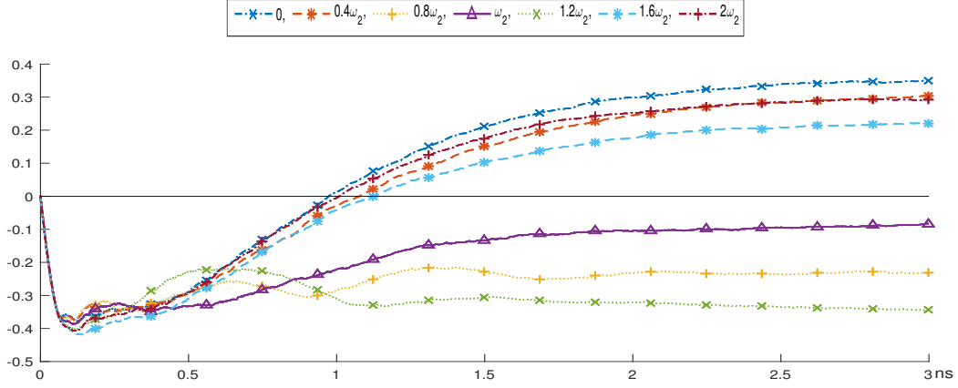
Figure 4: Consider System 4 with d = 100 . We show the Mandel-Q parameter (23) for different values of \omega_3 obtained from 20000 observations of Scheme 1. We take \omega_3 equal to 0, 0.4\omega_2 , 0.8\omega_2 , \omega_2 , 1.2\omega_2 , 1.6\omega_2 and 2\omega_2 .
